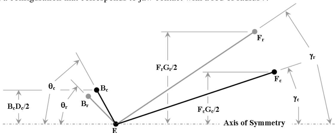
Figure 7: Stick diagram of member BEF in closed and partially open configurations
