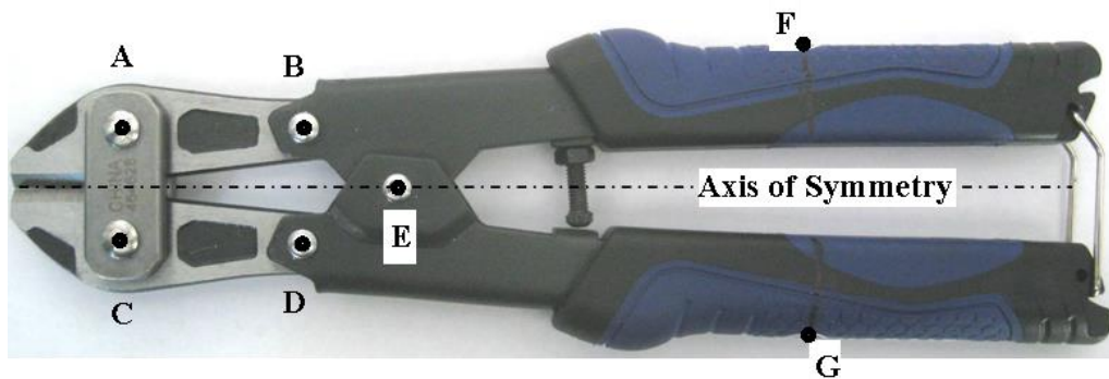
Figure 1: Image of 8" bolt cutter with labels for pins and operator input locations
