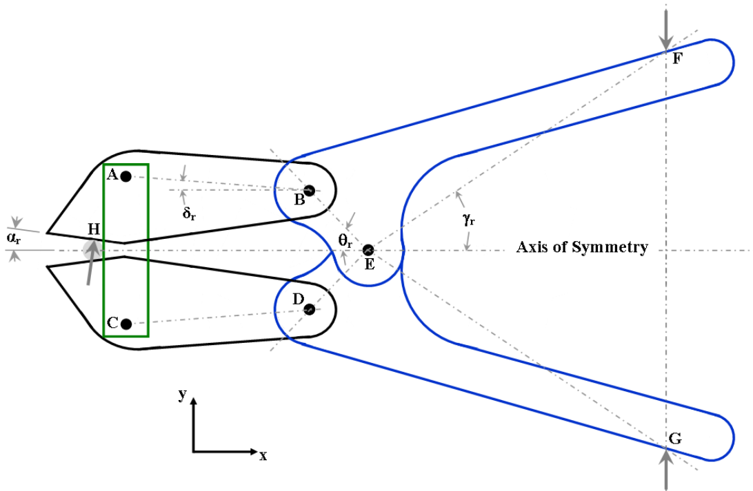
Figure 6: Bolt cutter diagram with labels for pin joints, force input locations, and angles Dimensions that must be determined include constant values such as the distance between pin joints that are on the same member, and non-constant values such as the relative angles between pin joints that vary with handle position. Constant values include distances AC, AB, BE, and BF. The varying relative angles between members ( \gamma , \theta , and \delta ) can be determined from pin to pin distances between pins on different members while the tool is in a configuration of interest. It is convenient to determine the varying angles \gamma , \theta , and \delta in the closed position ( \gamma_c , \theta_c , and \delta_c ) as well as for the configuration in which the jaws contact a rod of radius r ( \gamma_r , \theta_r , and \delta_r ). The author chose to rely on distance measurements to determine angular measurements since use of a protractor to measure angles on the tool proved cumbersome.
