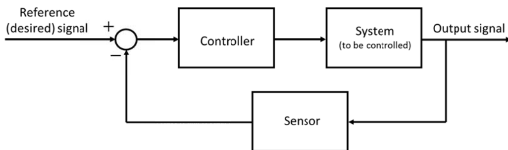
Figure 1: Classical feedback control loop showing a physical system to be controlled (“System”), its physical output, the desired plant output (“Reference (desired) signal”), and the controller that achieves the desired objectives.
