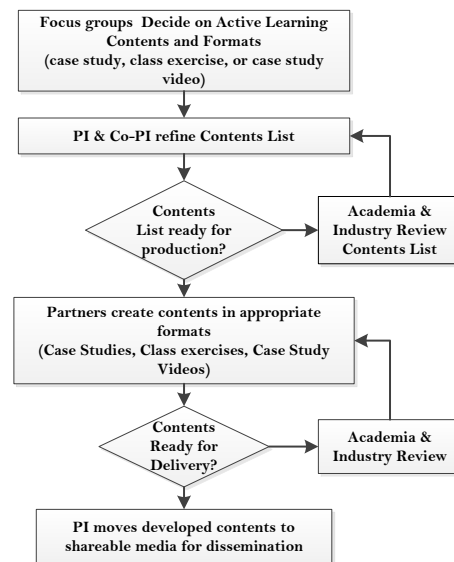
Figure 1: Development Methodology
