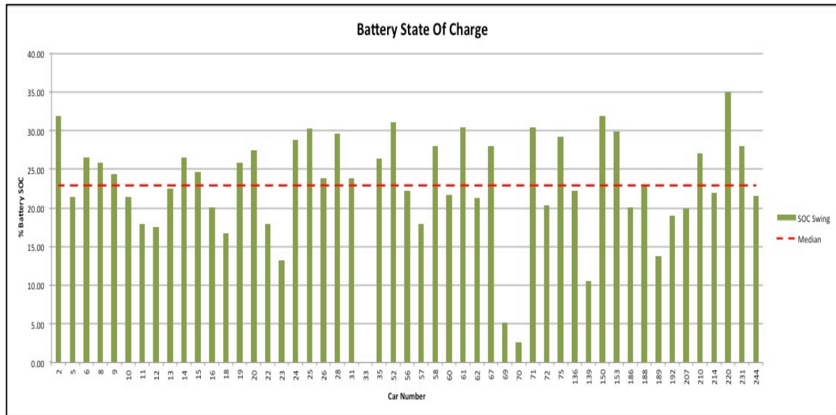
Figure 4: The battery usage trend among all the EVs
