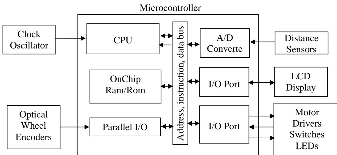
Figure 2. Microcontroller-based micromouse system
