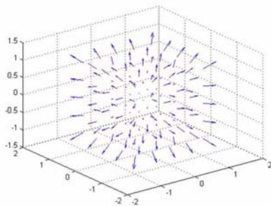
(a) Vector field
