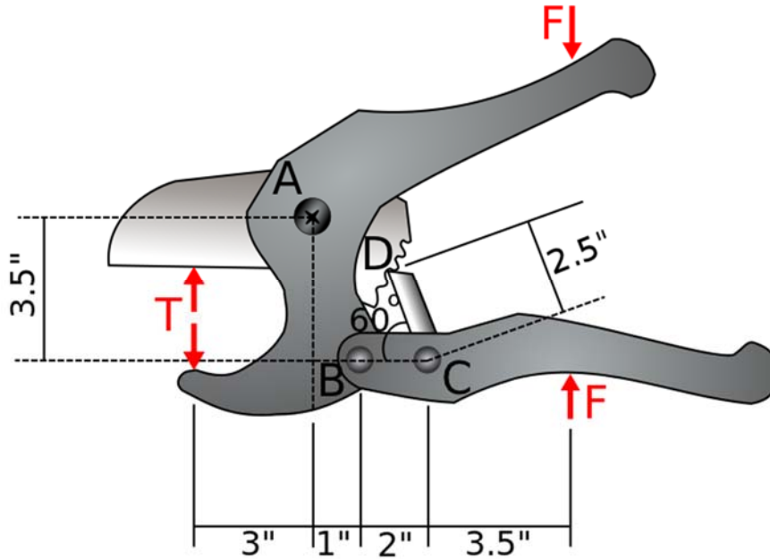
Figure 1: Typical problem from the Statics course. The problem statement reads as follows, “The device shown is used for cutting PVC pipe. If a force, F = 15 lb., is applied to each handle as shown, determine the cutting force T . Also, determine the magnitude and the direction of the force that the pivot at A applies to the blade.”
