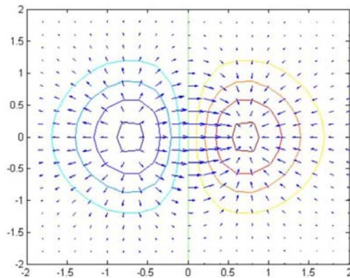
(b) Gradient and Countours of Function
