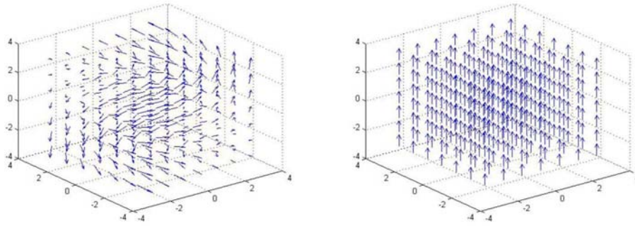
(a) Vector Field
