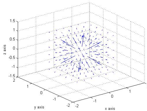
Figure 7: Electric Field of a unit charge.
