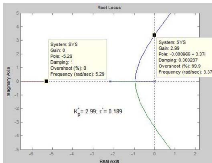
Figure 7. Root locus of a third order system with critical gain K_p=3 .
