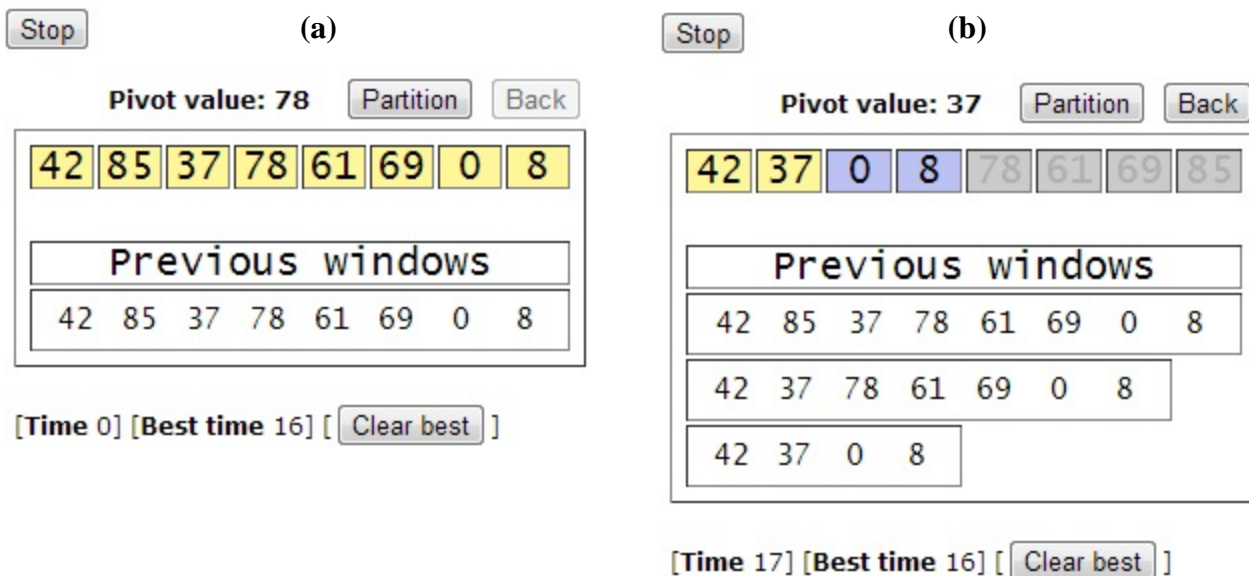
Figure 5: Quick sorter activity intuitively teaches the quick sort algorithm. (a) The student must select all values in the current window of values that are smaller than the pivot value, then click the "Partition" button. Highlighted values are blue, while unhighlighted are yellow. (b) The previous windows are displayed to visualize the recursion.
