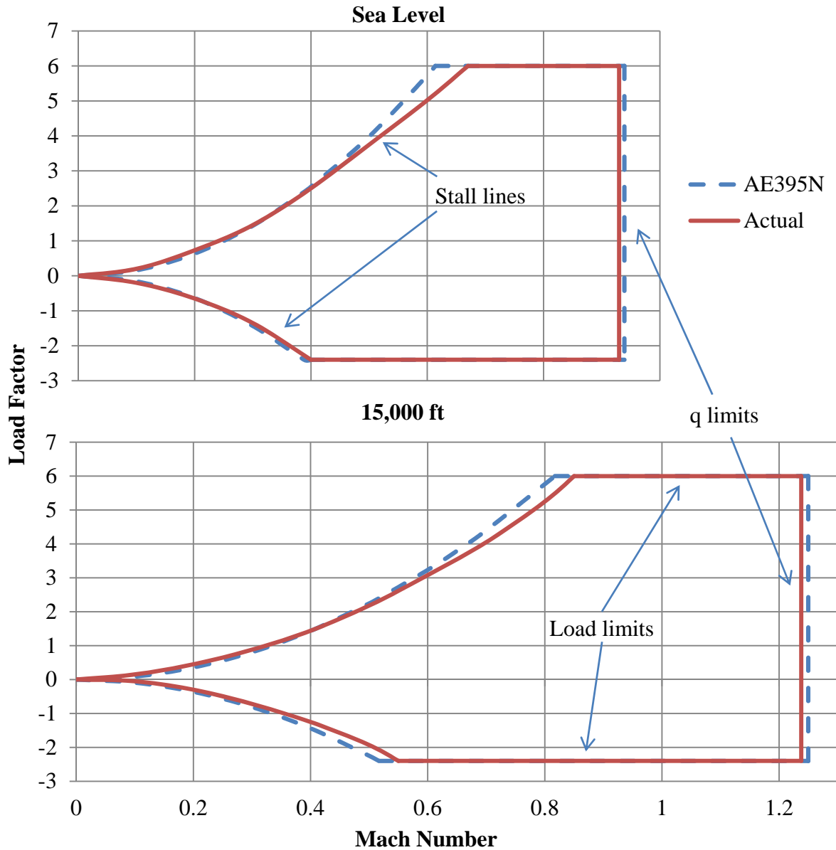
Figure 6: V-n Diagrams
