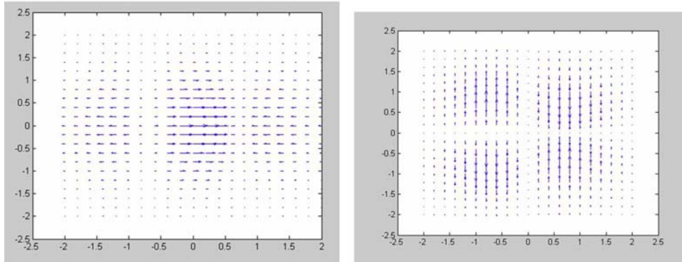
(c) Directional Derivative in \vec{a}_x direction (d) Directional Derivative in \vec{a}_y direction
