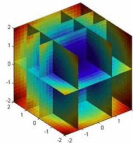
(b) Divergence (Flux) of Vector Field
